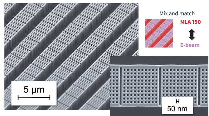
Mix-and-match lithography
